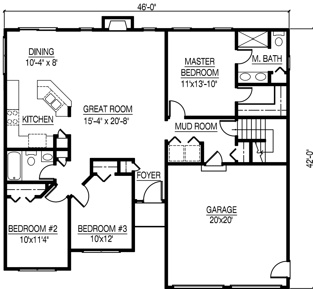
FLOOR PLAN
